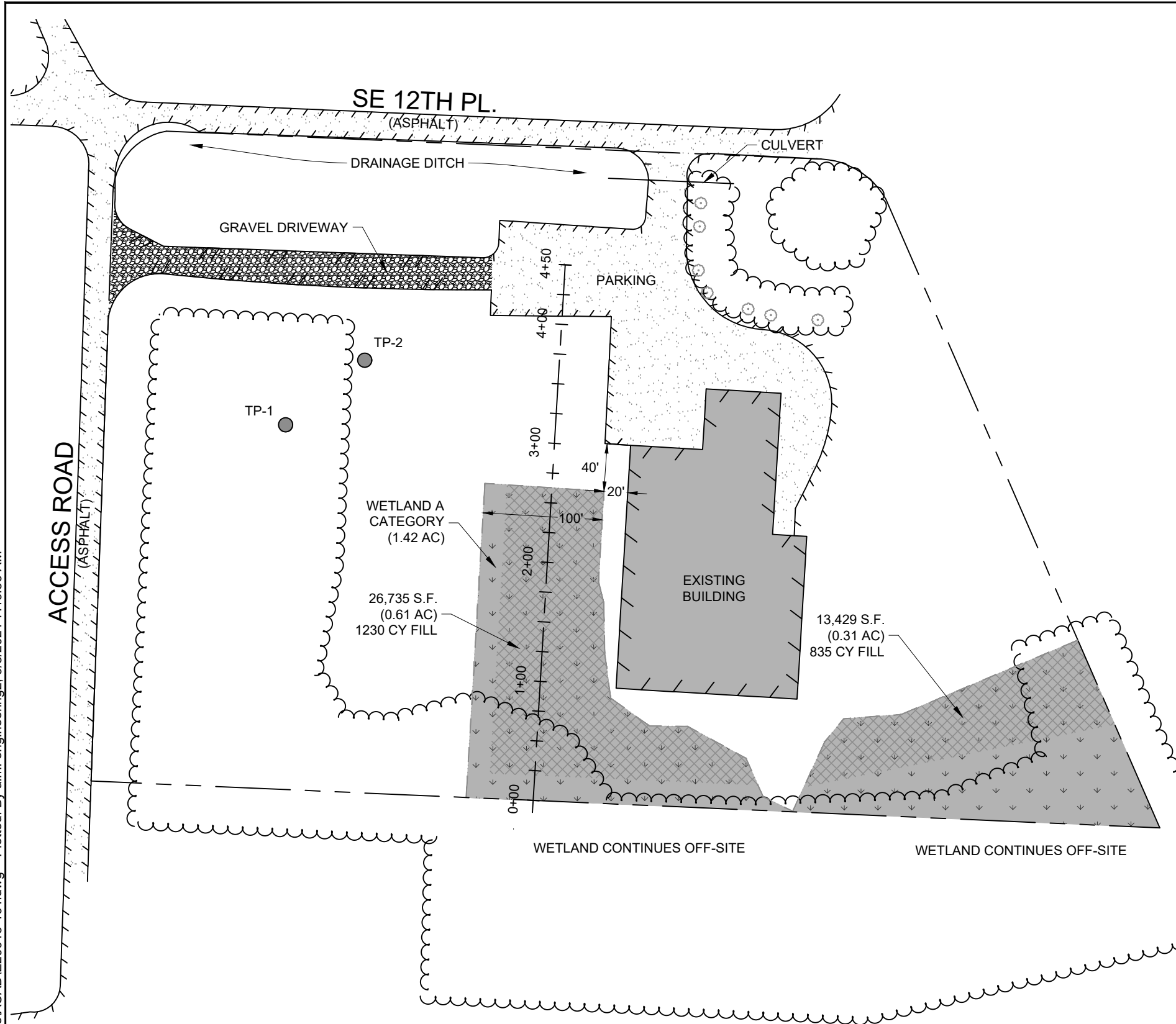
FIGURE 2, SITE MAP
